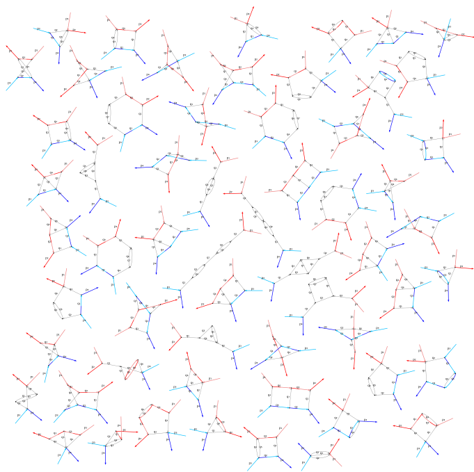
All scaleful diagrams, in the classical limit at 2 loops in GR
