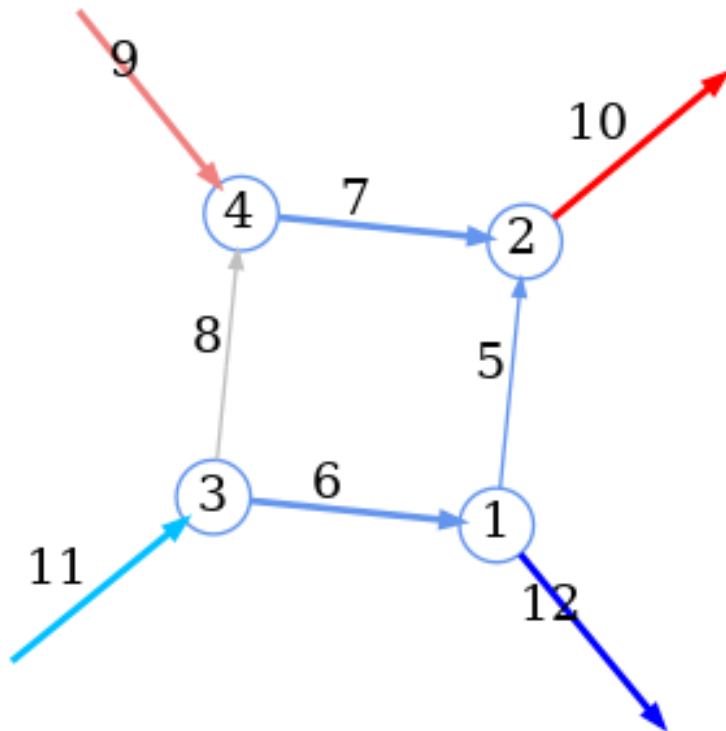
Fig 5.2: The maximal mass spanning tree of the box diagram in blue. The loop momenta are the edges that are missing from the tree.
