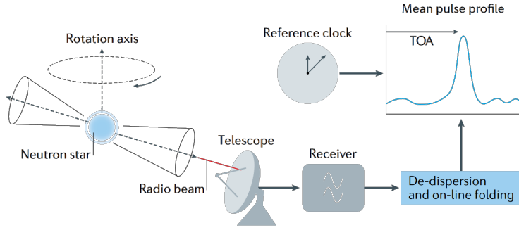
Fig 3.5: How pulsar timing arrays work
