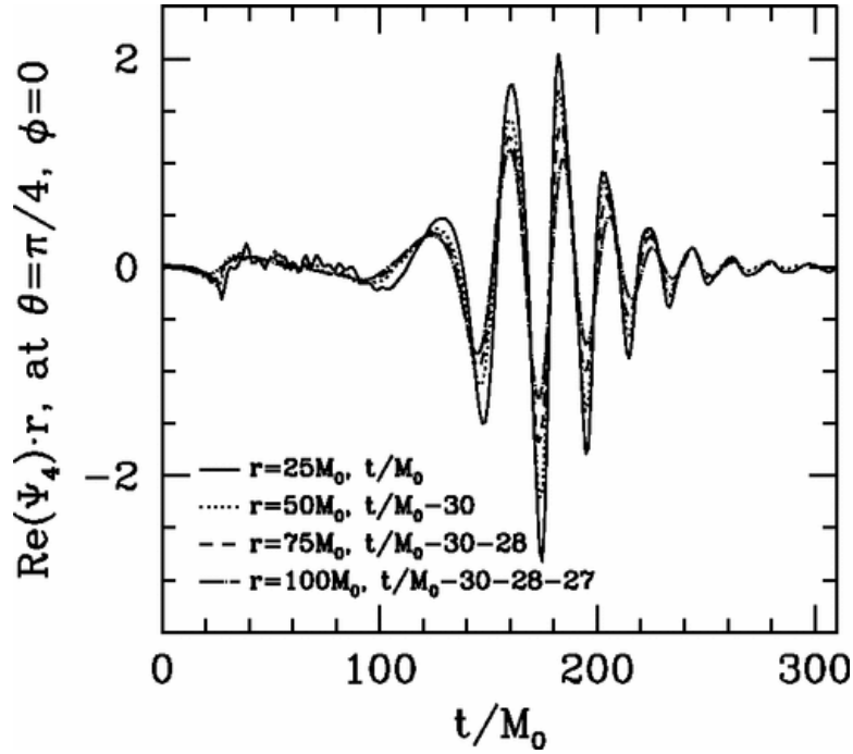
Fig 4.2: The first NR waveform, as presented in [25]
