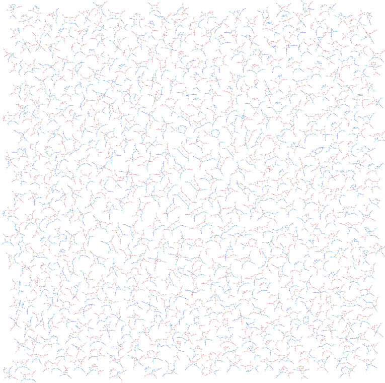
All scaleful diagrams, in the classical limit at two loops in SQED
