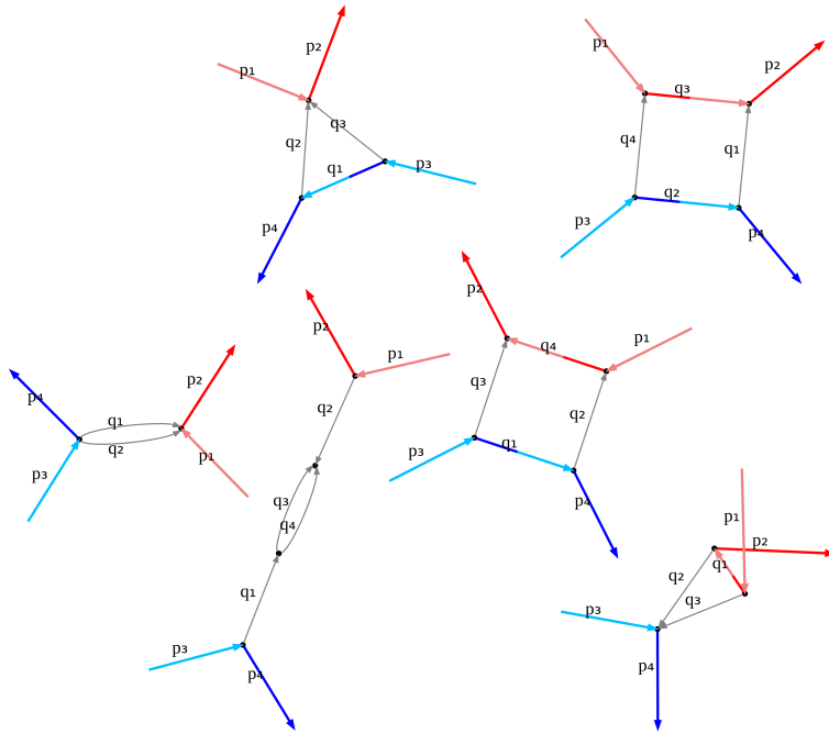
All scaleful diagrams, in the classical limit at 1 loop in GR
