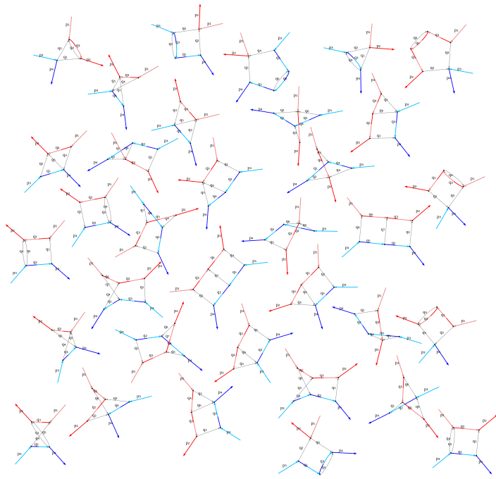
All scaleful diagrams, in the classical limit at two loops in SQED
