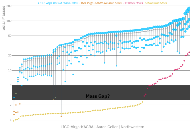
Fig 3.3: Mass distribution of Detected GW emitting binaries. Credit: Visualization: LIGO-Virgo-KAGRA / Aaron Geller / Northwestern
