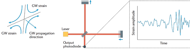
Fig 3.1: Principles of laser interferometer GW detectors
